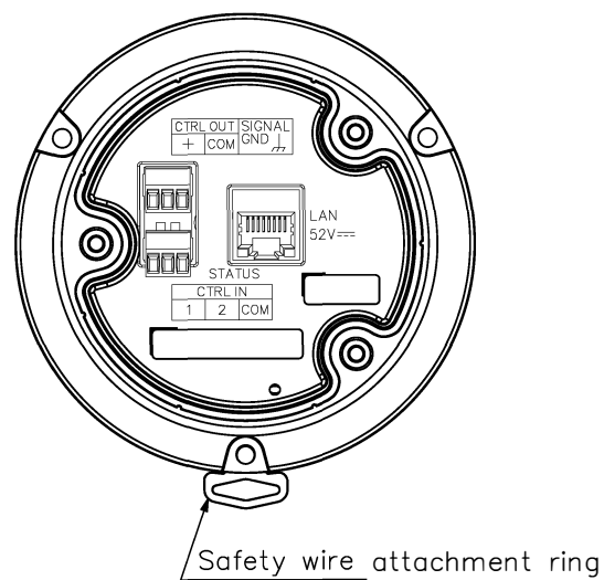
Close-up with rear cover removed
